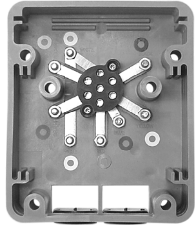
3850031 SMART BOX Adapter
